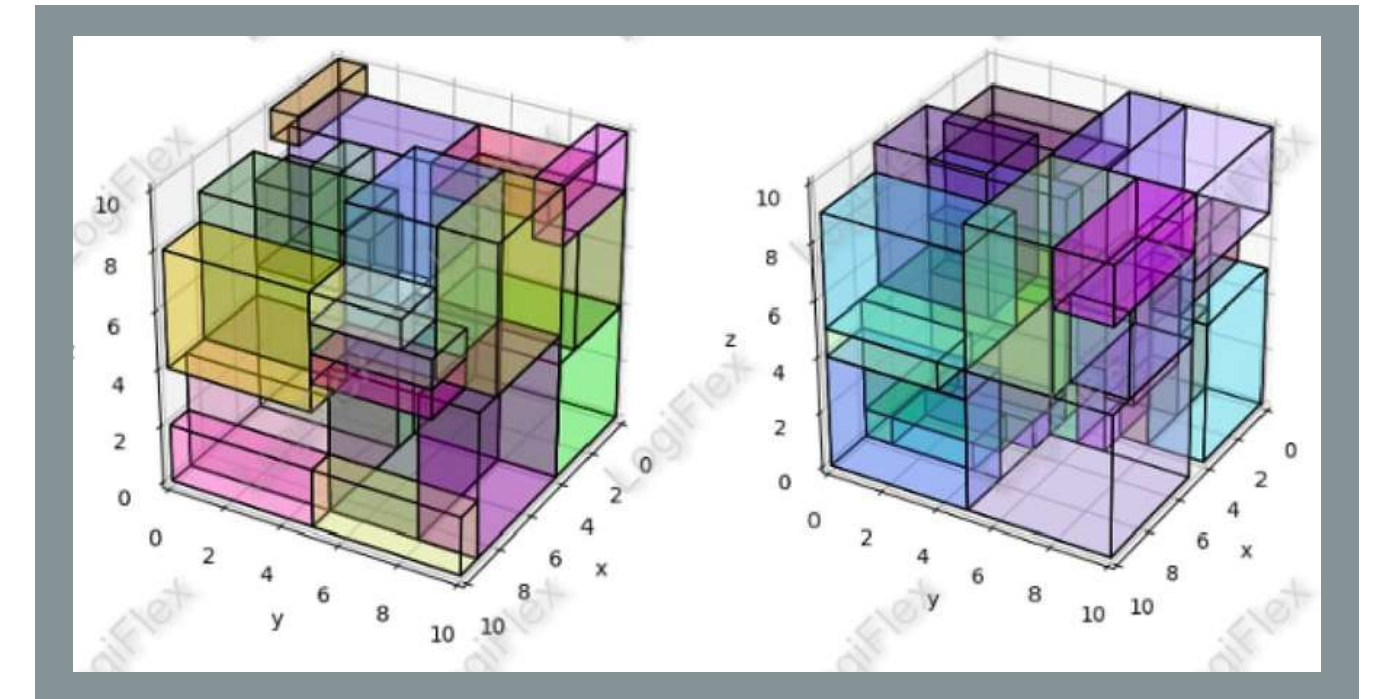
optimal algorithm
